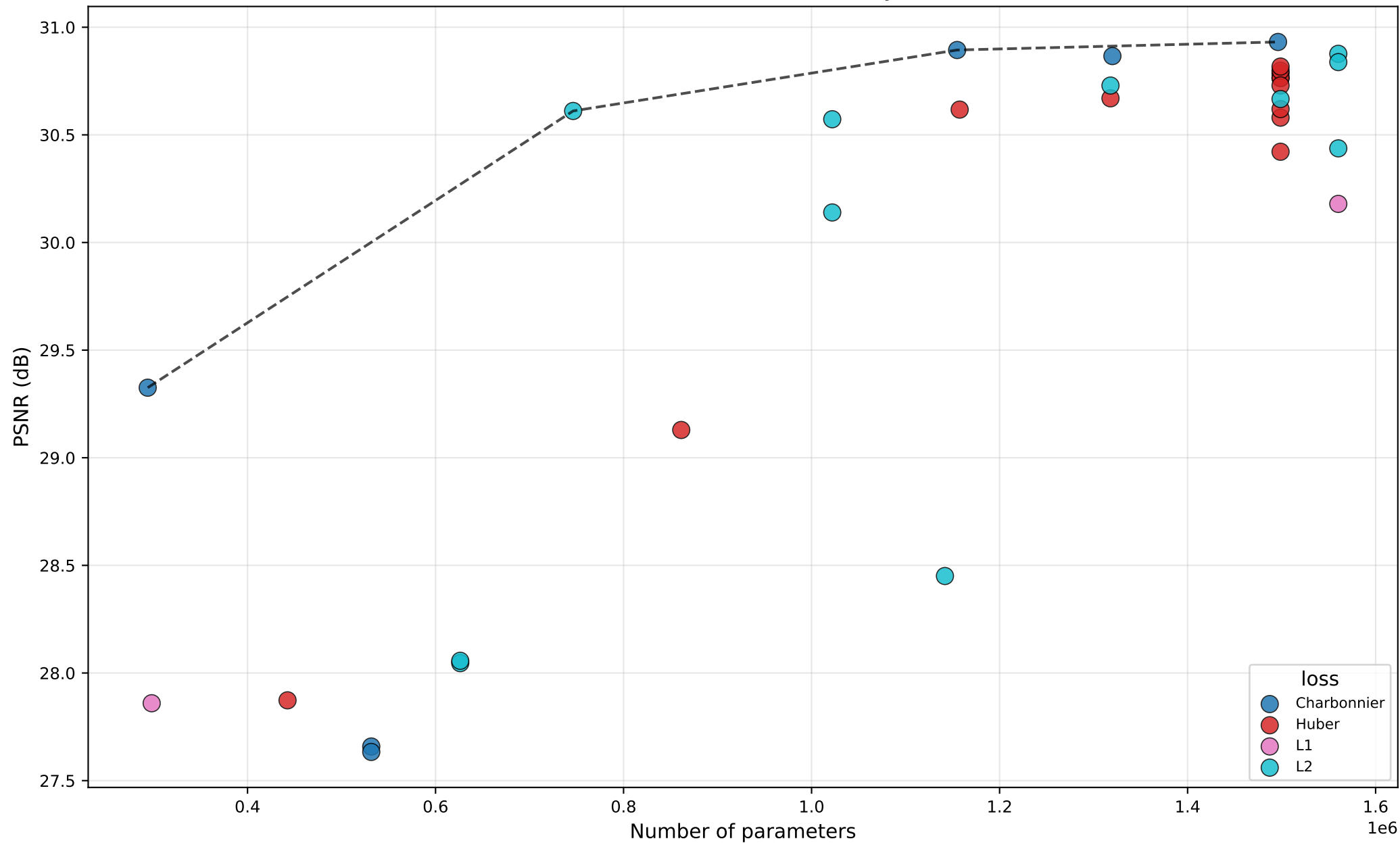
PSNR vs #Params — DAT — by loss
